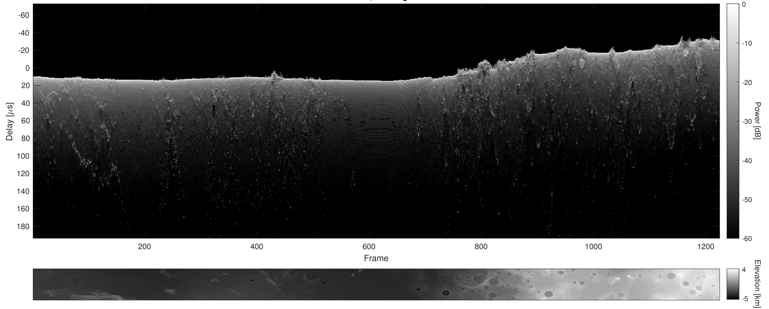
Orbit 7181, Cluttergram
