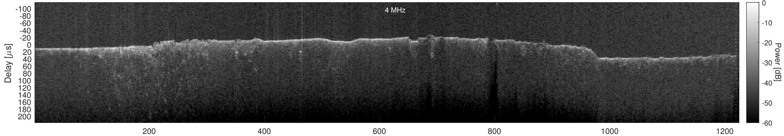
Orbit 7182, Cluttergram
