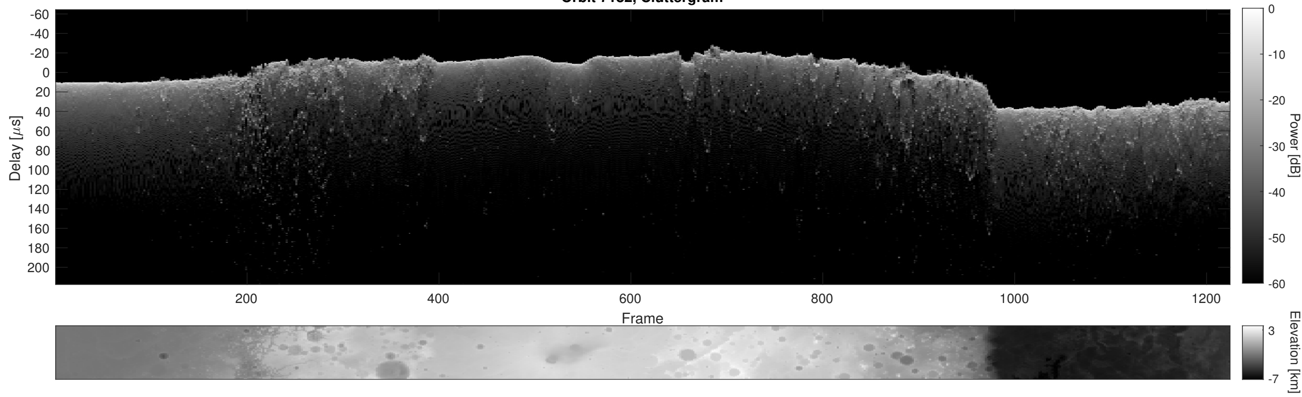
Orbit 7182, Cluttergram
