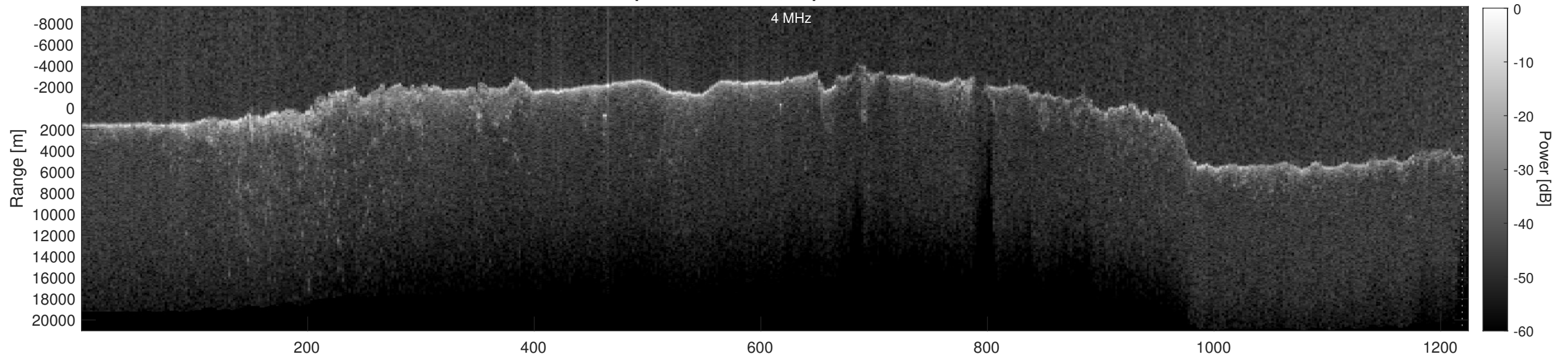
Orbit 7182, Depth-Corrected Cluttergram
