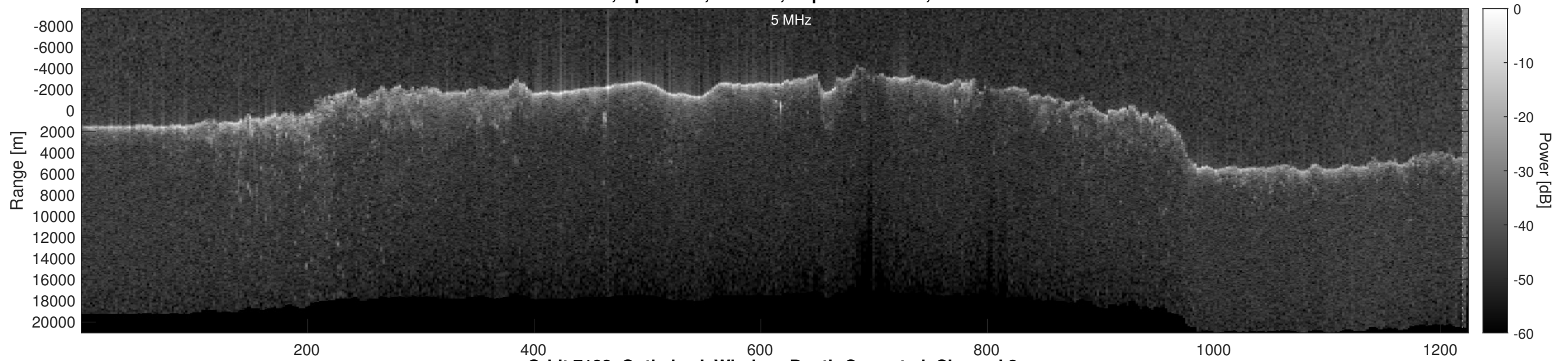
Orbit 7182, Optimized, Window, Depth-Corrected, Channel 2
