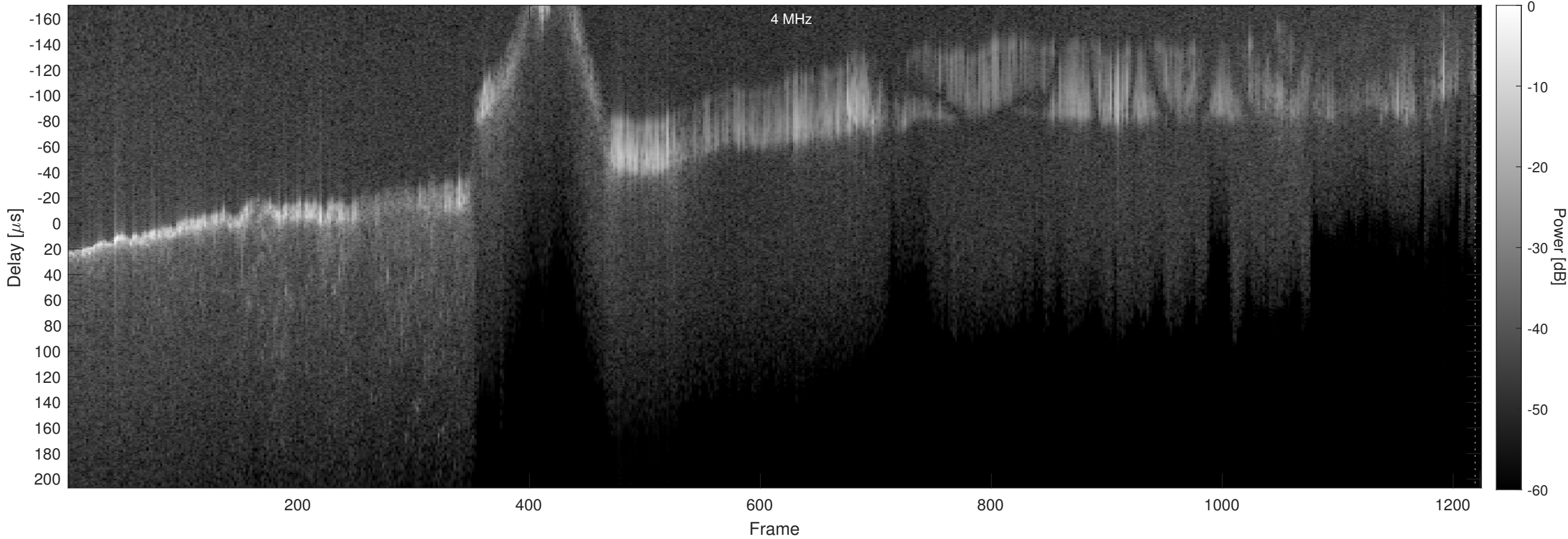
Orbit 7184, Chapman, No Window, Channel 2
