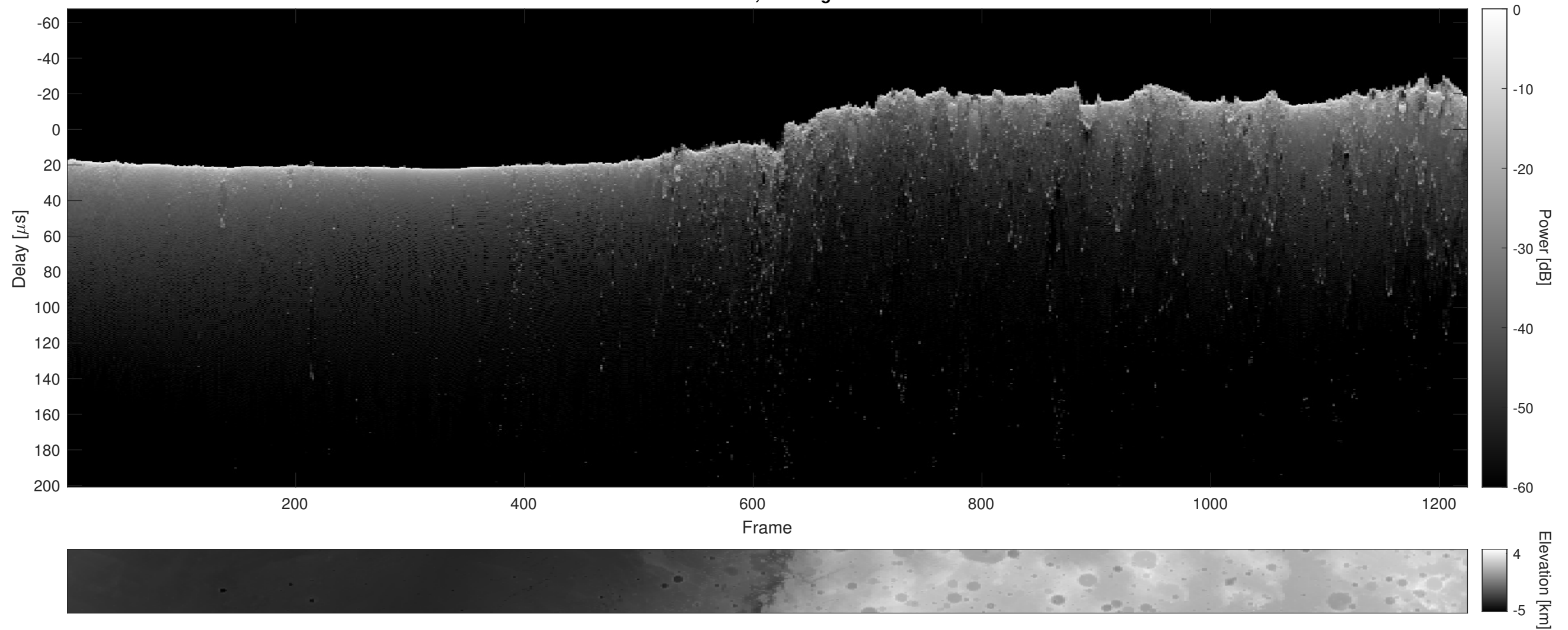
Orbit 7185, Cluttergram
