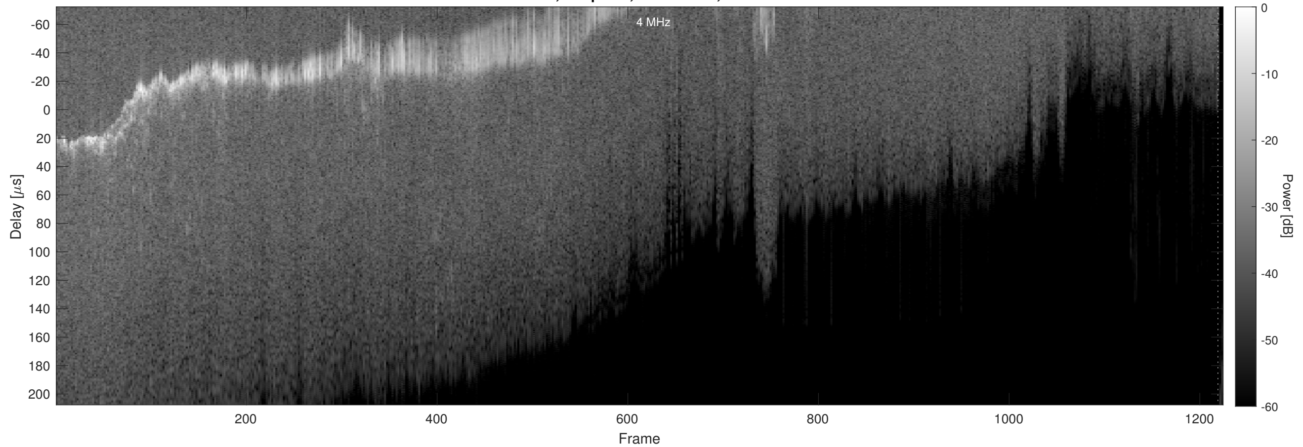
Orbit 7187, Chapman, No Window, Channel 2
