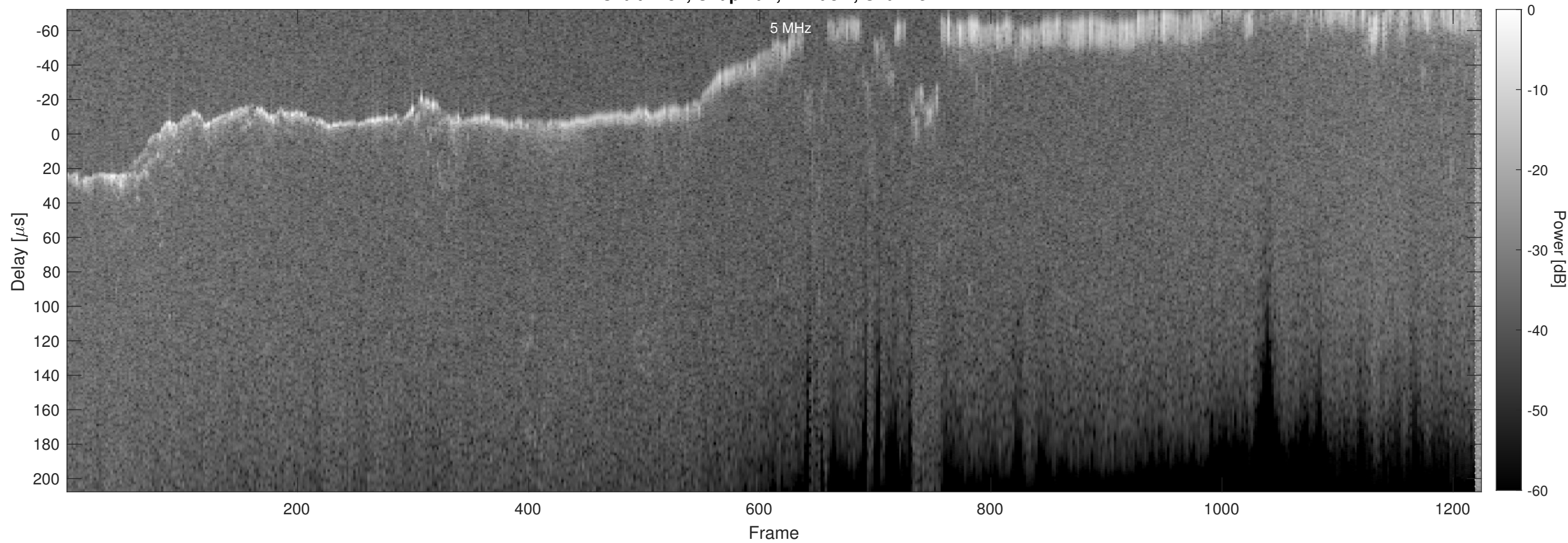
Orbit 7187, Chapman, Window, Channel 2
