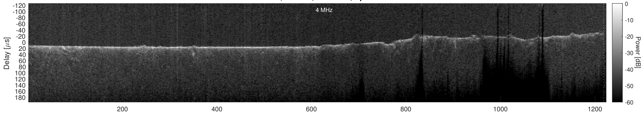
Orbit 7188, Cluttergram
