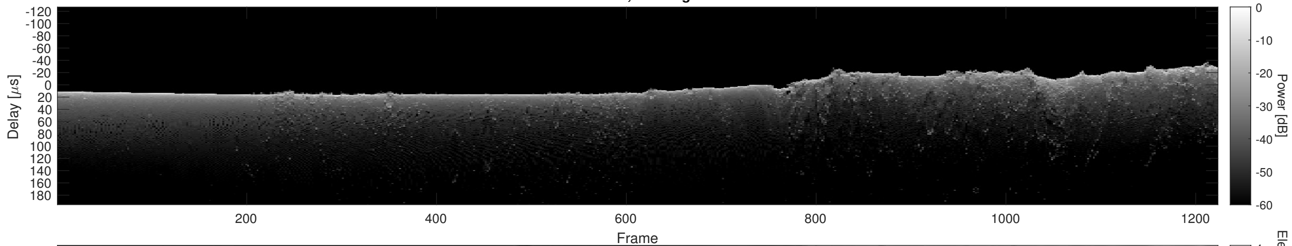
Orbit 7188, Cluttergram
