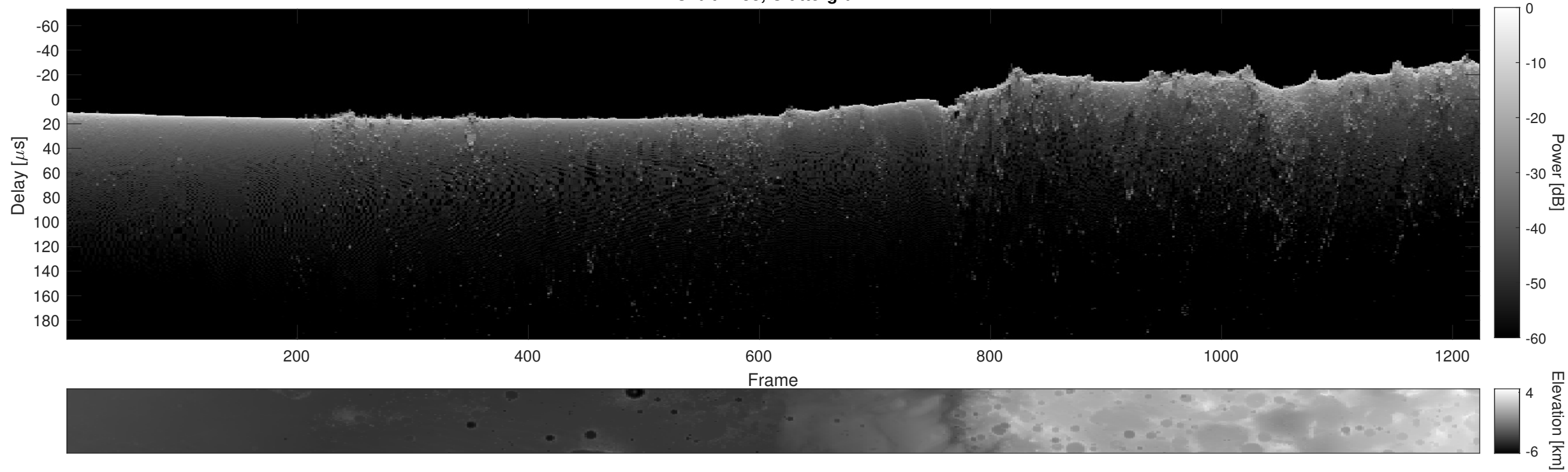
Orbit 7188, Cluttergram
