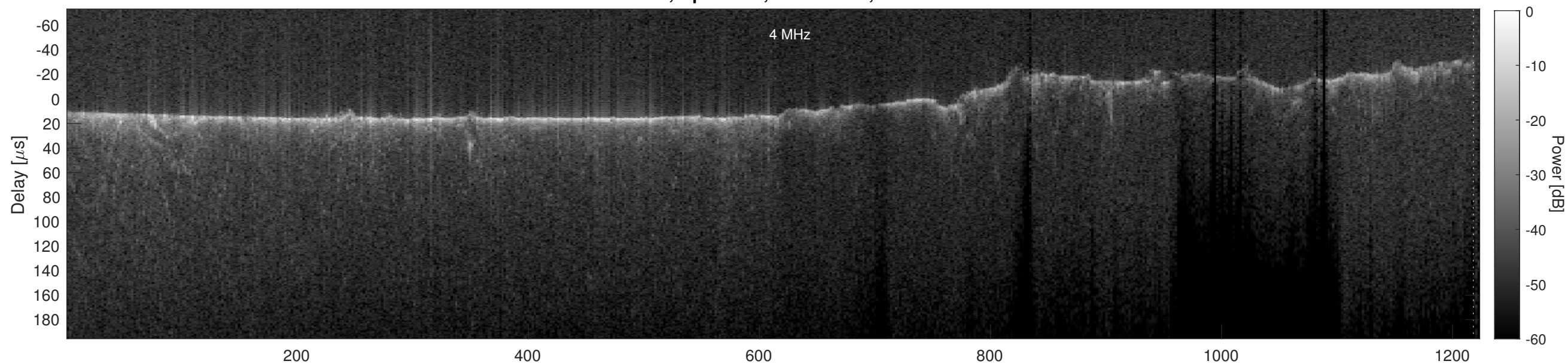
Orbit 7188, Cluttergram
