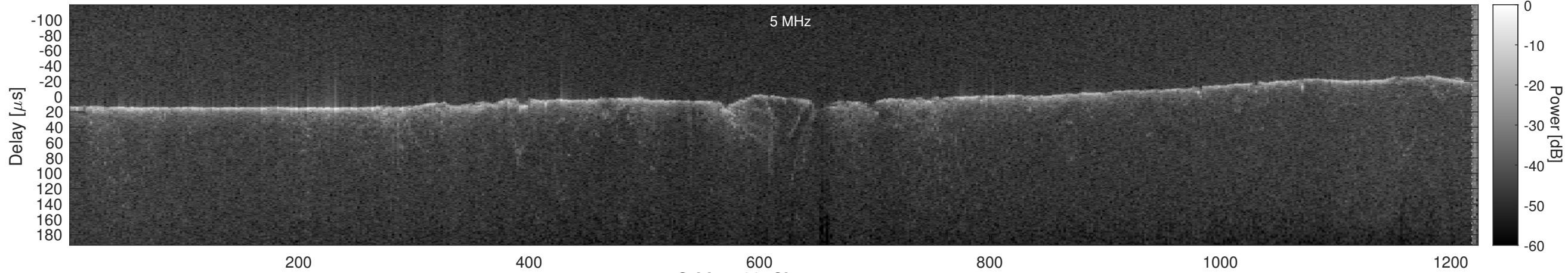
Orbit 7190, Cluttergram
