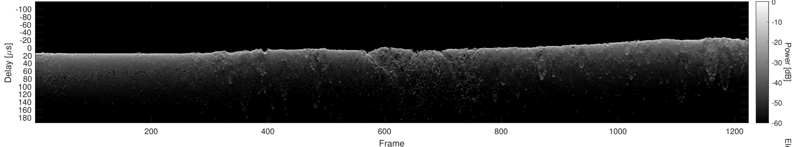
Orbit 7190, Cluttergram
