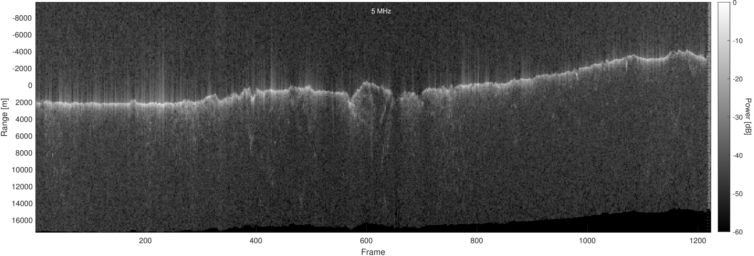
Orbit 7190, Optimized, No Window, Depth-Corrected, Channel 2
