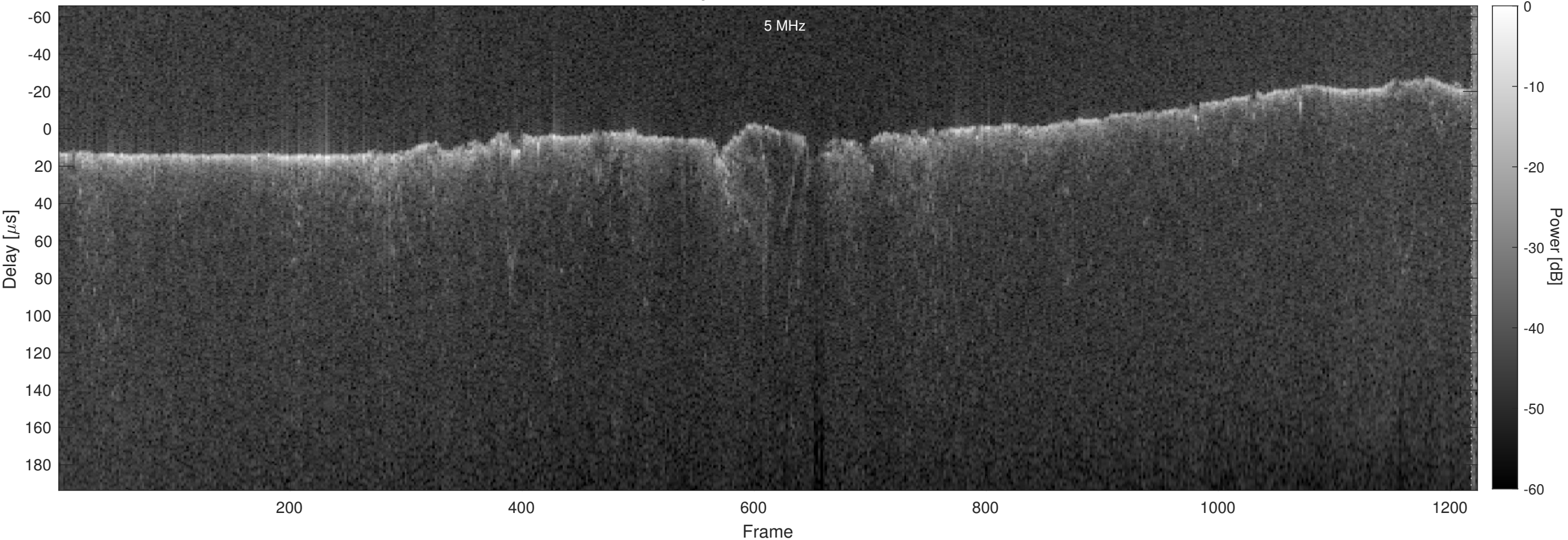
Orbit 7190, Optimized, Window, Channel 2
