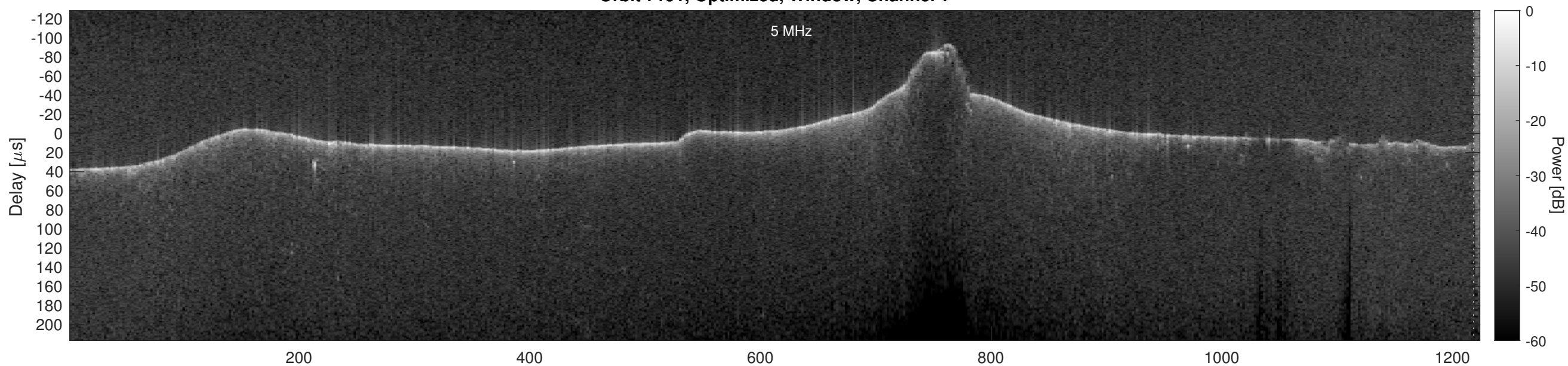
Orbit 7191, Optimized, Window, Channel 2
