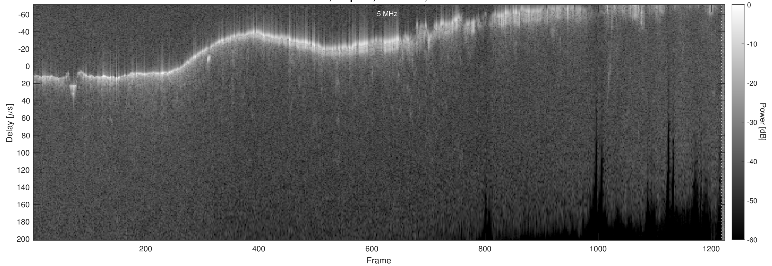
Orbit 7192, Chapman, No Window, Channel 2
