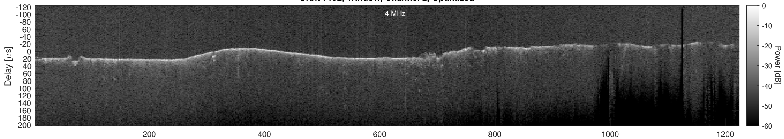
Orbit 7192, Cluttergram
