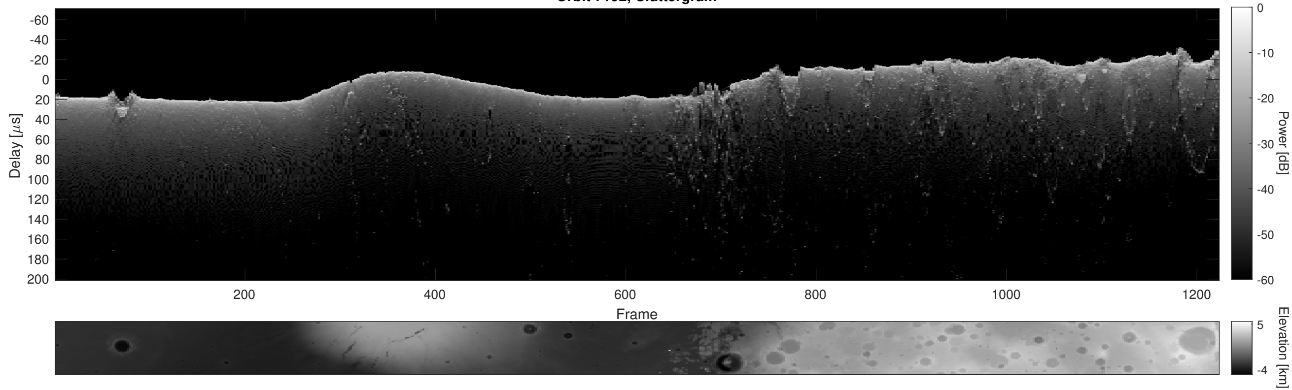
Orbit 7192, Cluttergram
