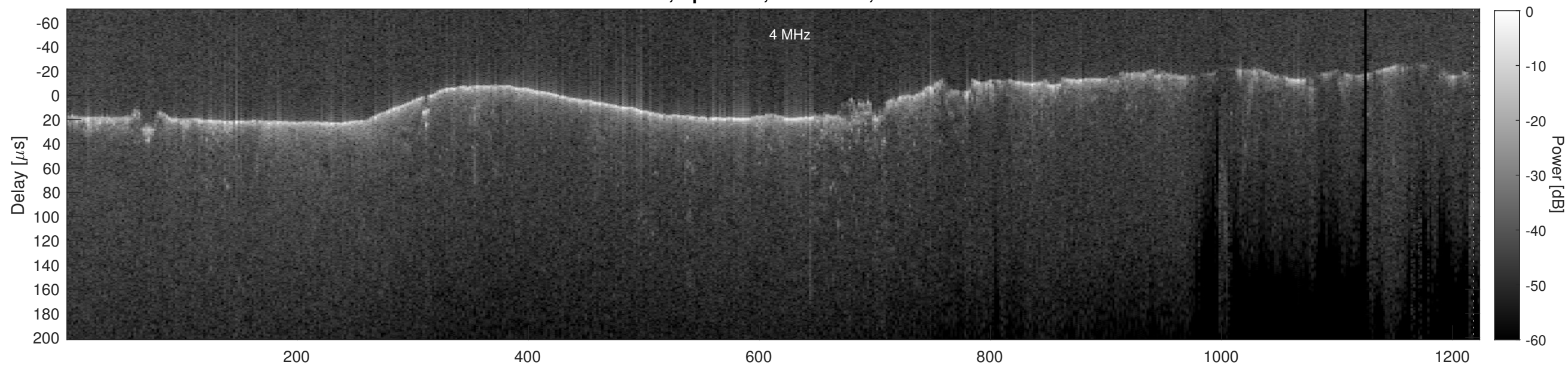
Orbit 7192, Cluttergram
