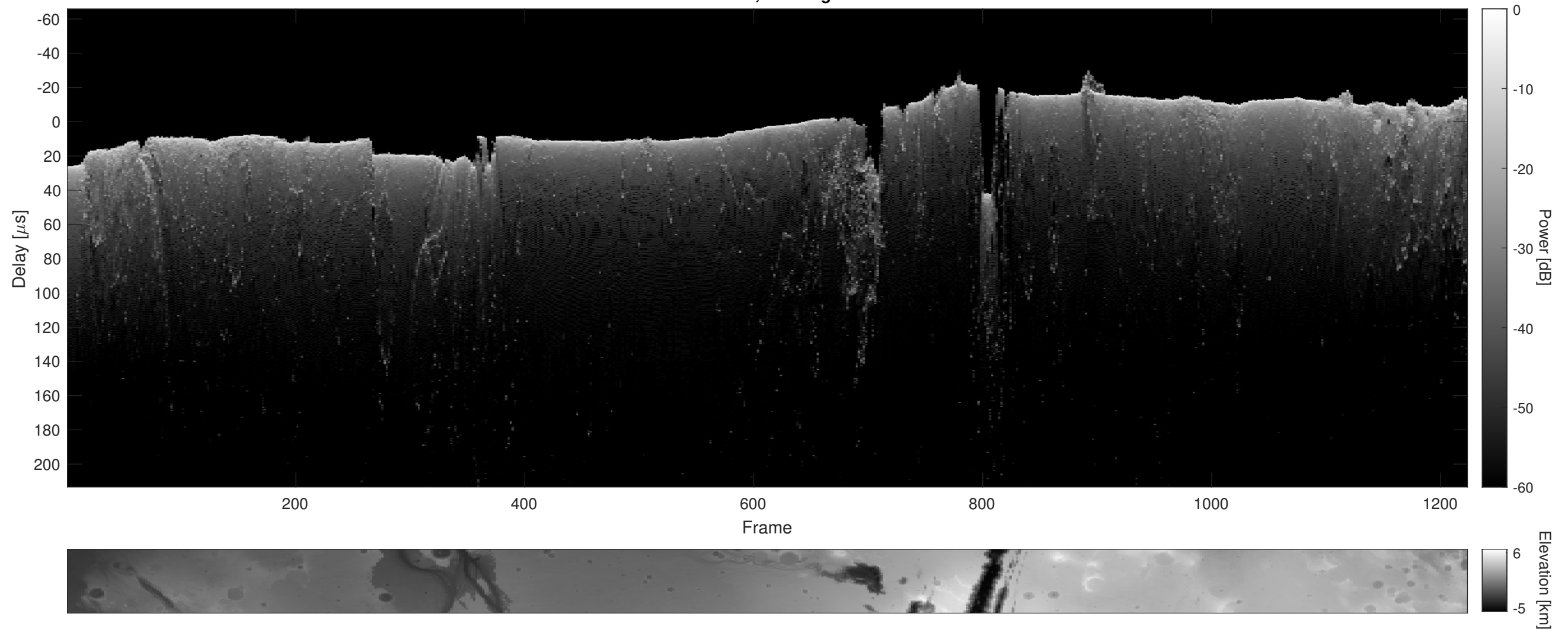
Orbit 7194, Cluttergram
