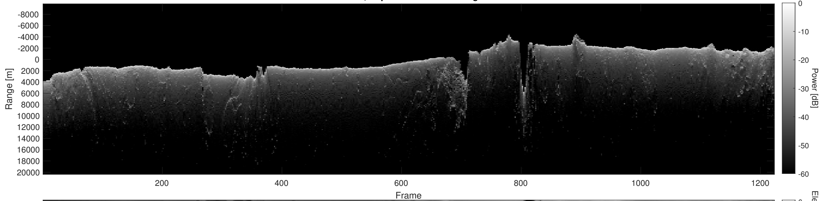
Orbit 7194, Depth-Corrected Cluttergram
