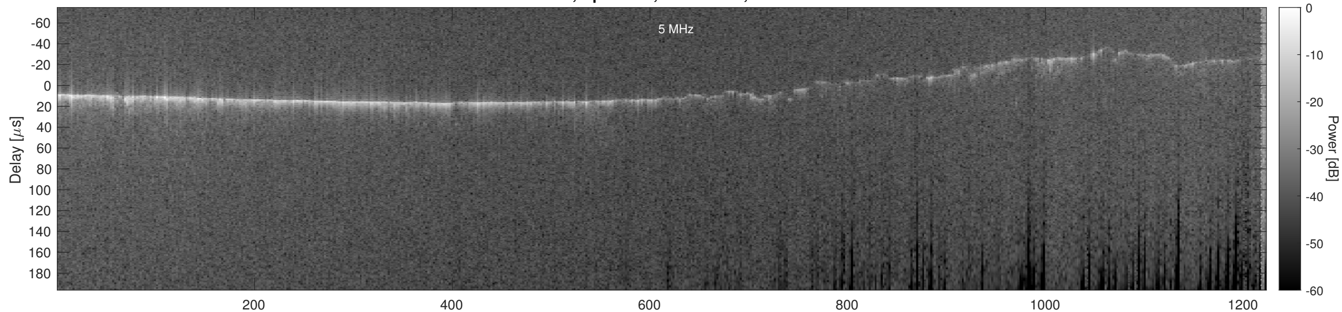
Orbit 7195, Optimized, No Window, Channel 2
