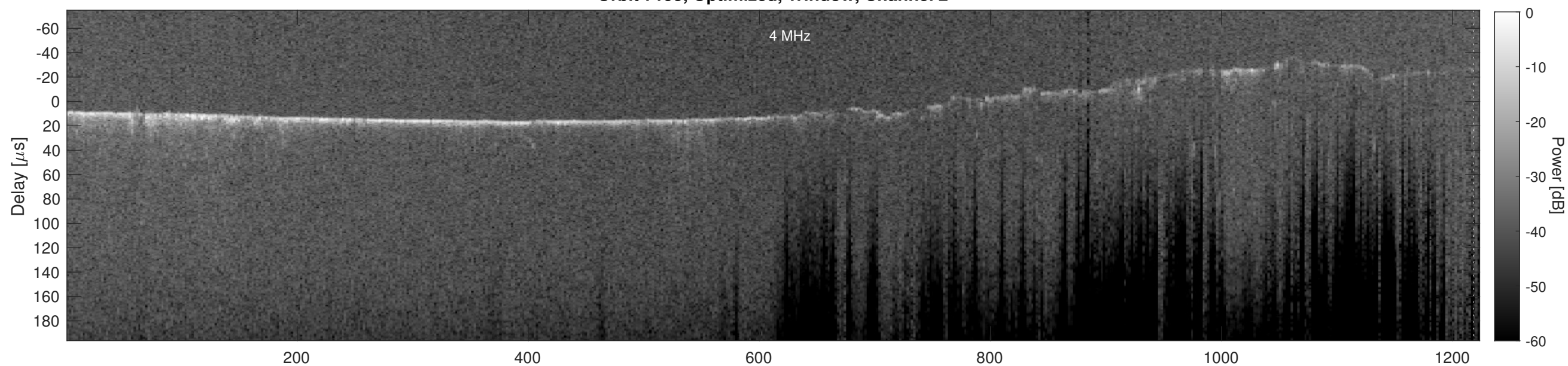
Orbit 7195, Cluttergram
