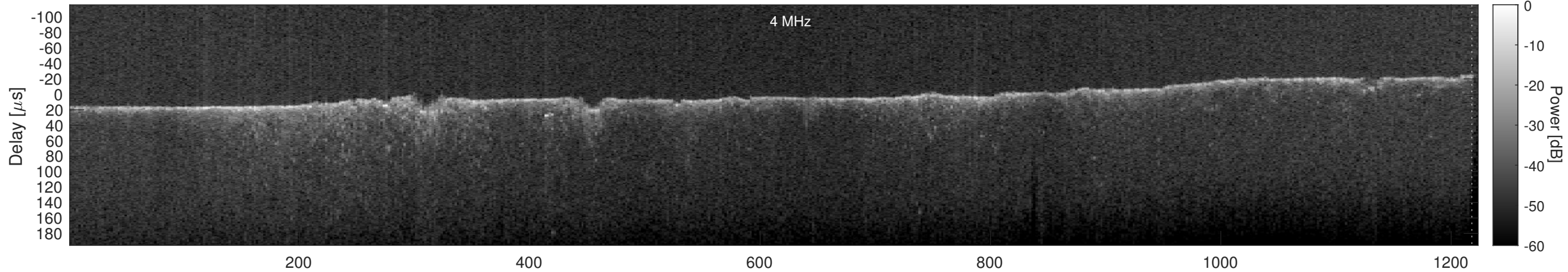
Orbit 7197, Cluttergram
