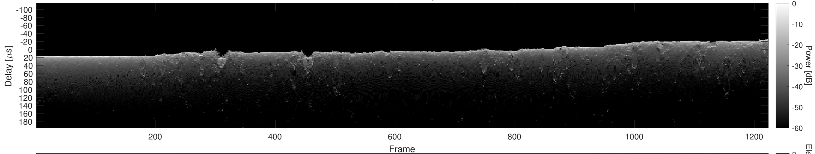
Orbit 7197, Cluttergram
