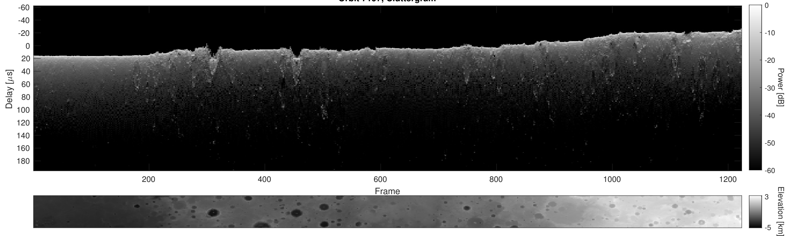
Orbit 7197, Cluttergram
