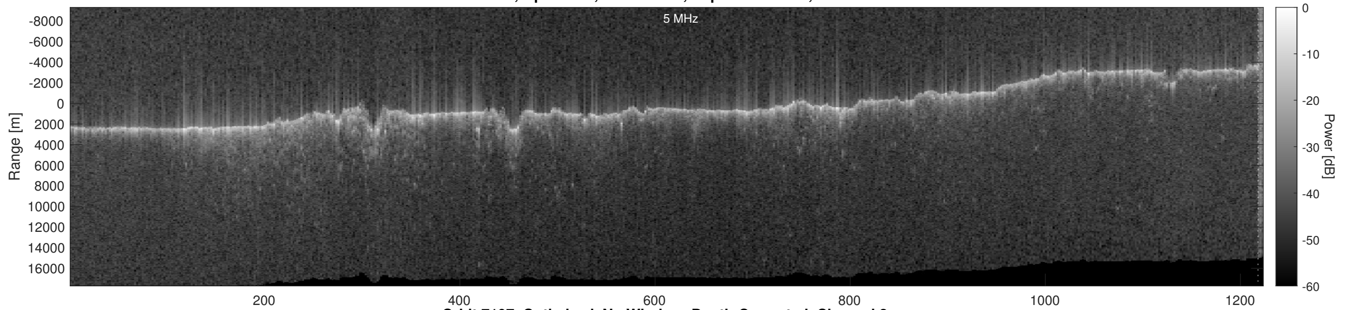
Orbit 7197, Optimized, No Window, Depth-Corrected, Channel 2
