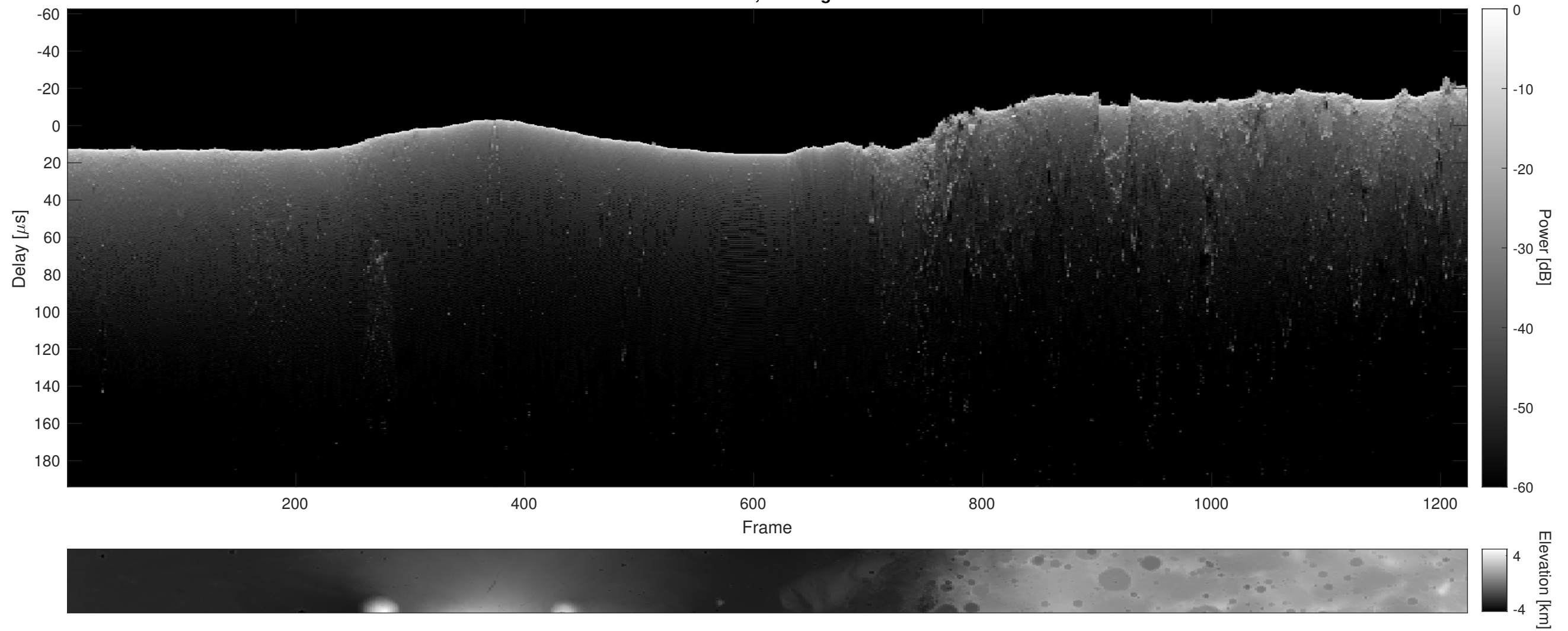
Orbit 7199, Cluttergram
