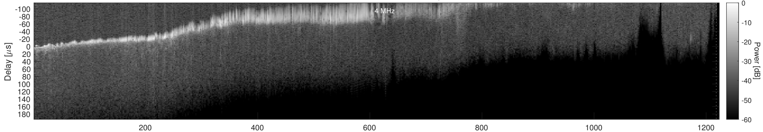
Orbit 7199, Window, Channel 2, Optimized
