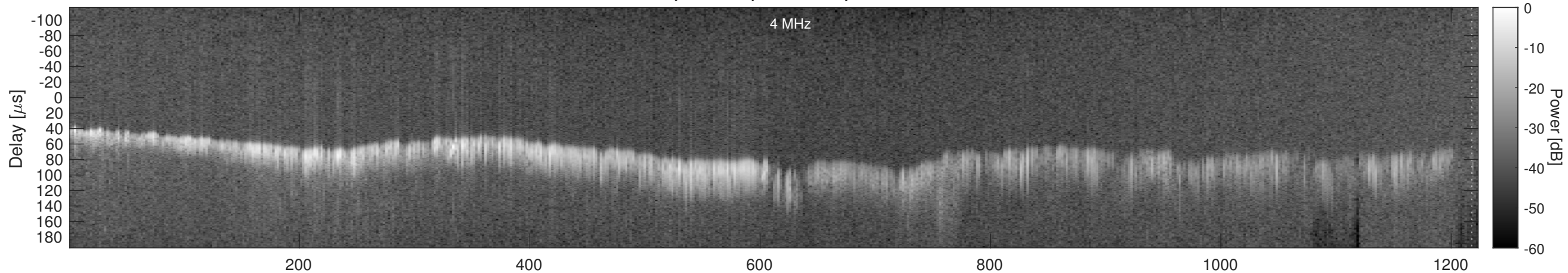
Orbit 7199, Window, Channel 2, Chapman
