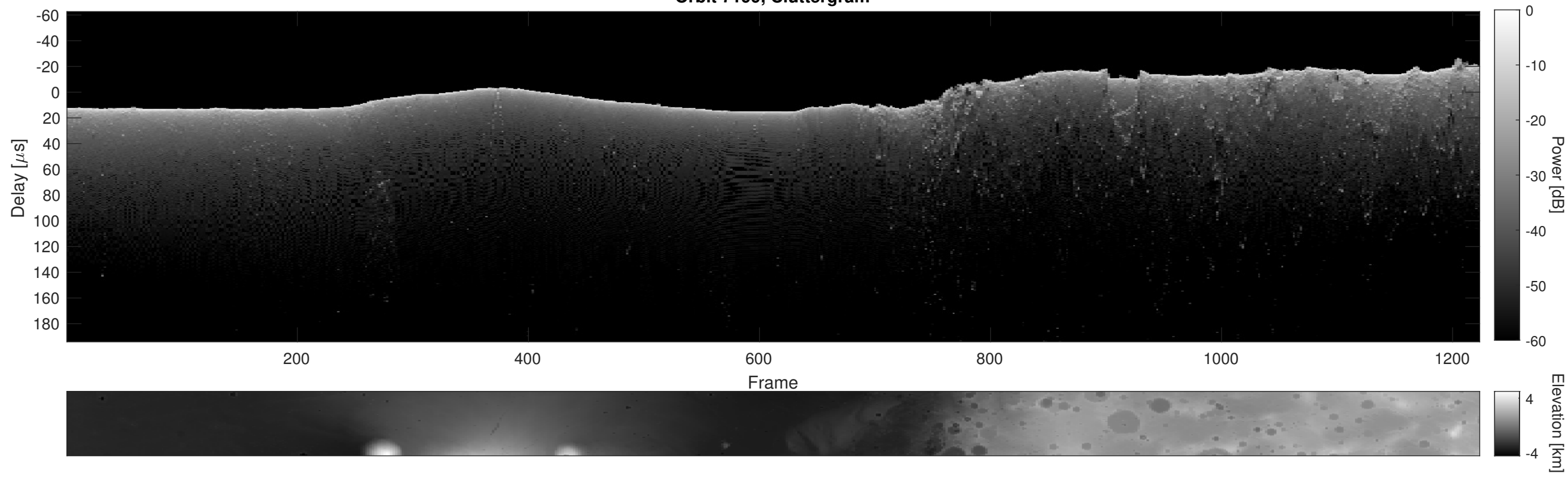
Orbit 7199, Cluttergram
