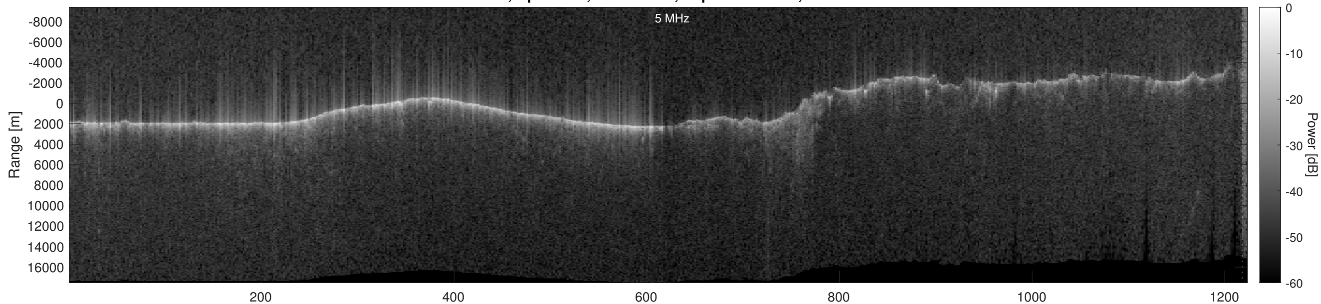
Orbit 7199, Optimized, No Window, Depth-Corrected, Channel 2
