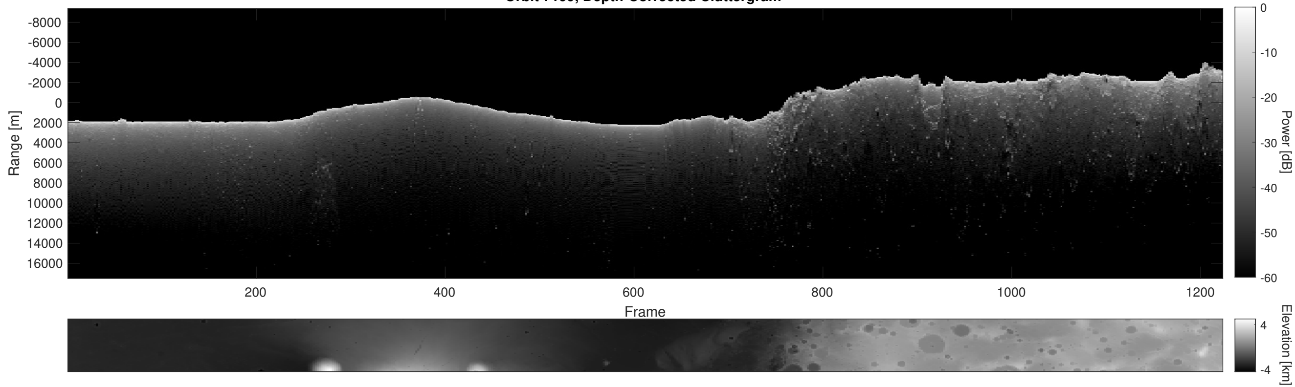
Orbit 7199, Depth-Corrected Cluttergram
