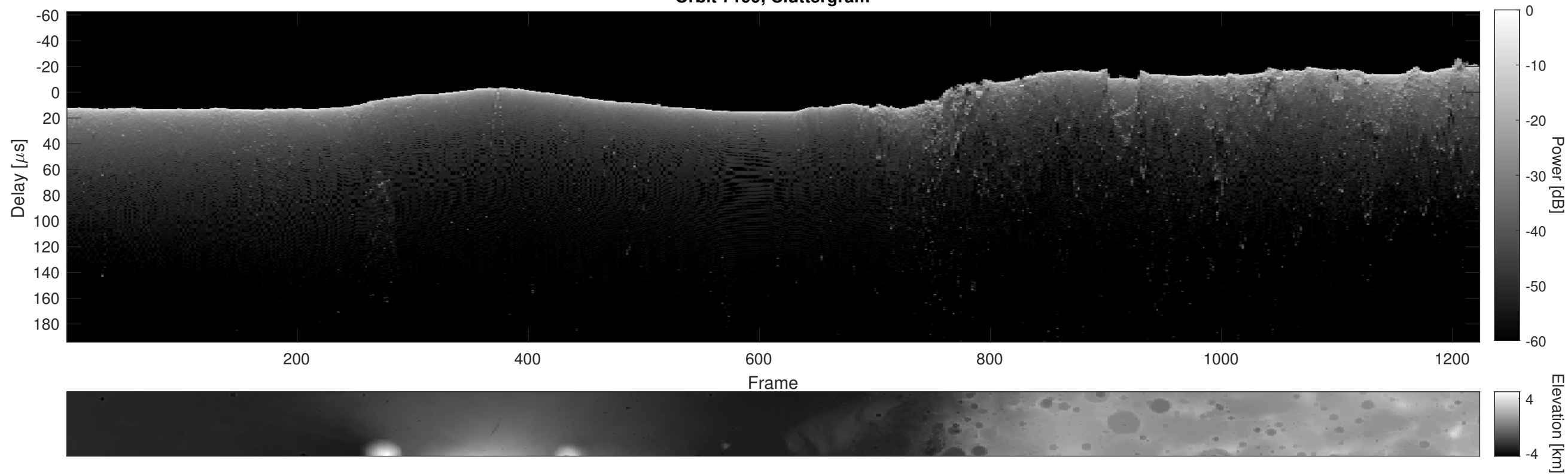
Orbit 7199, Cluttergram
