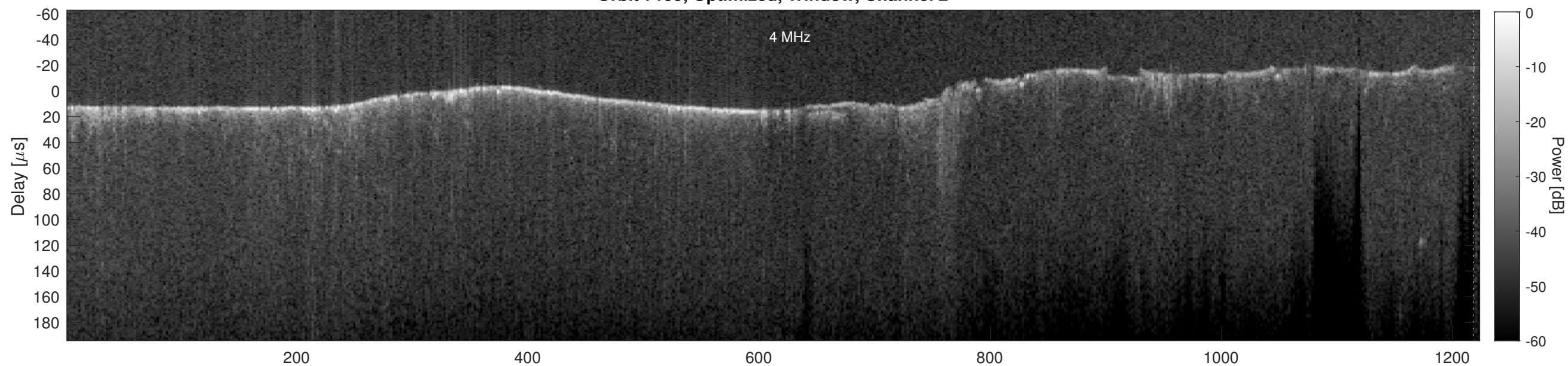
Orbit 7199, Cluttergram
