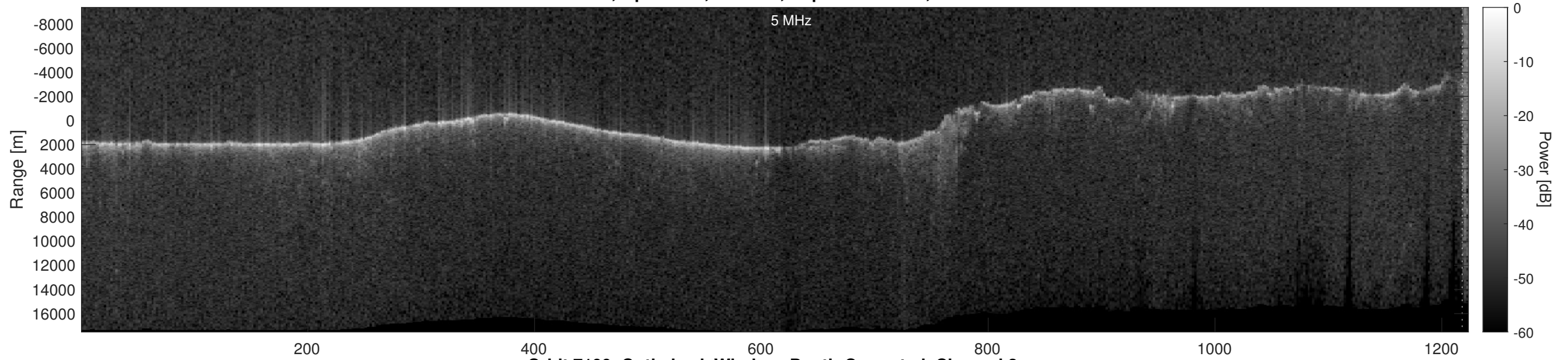
Orbit 7199, Optimized, Window, Depth-Corrected, Channel 2
