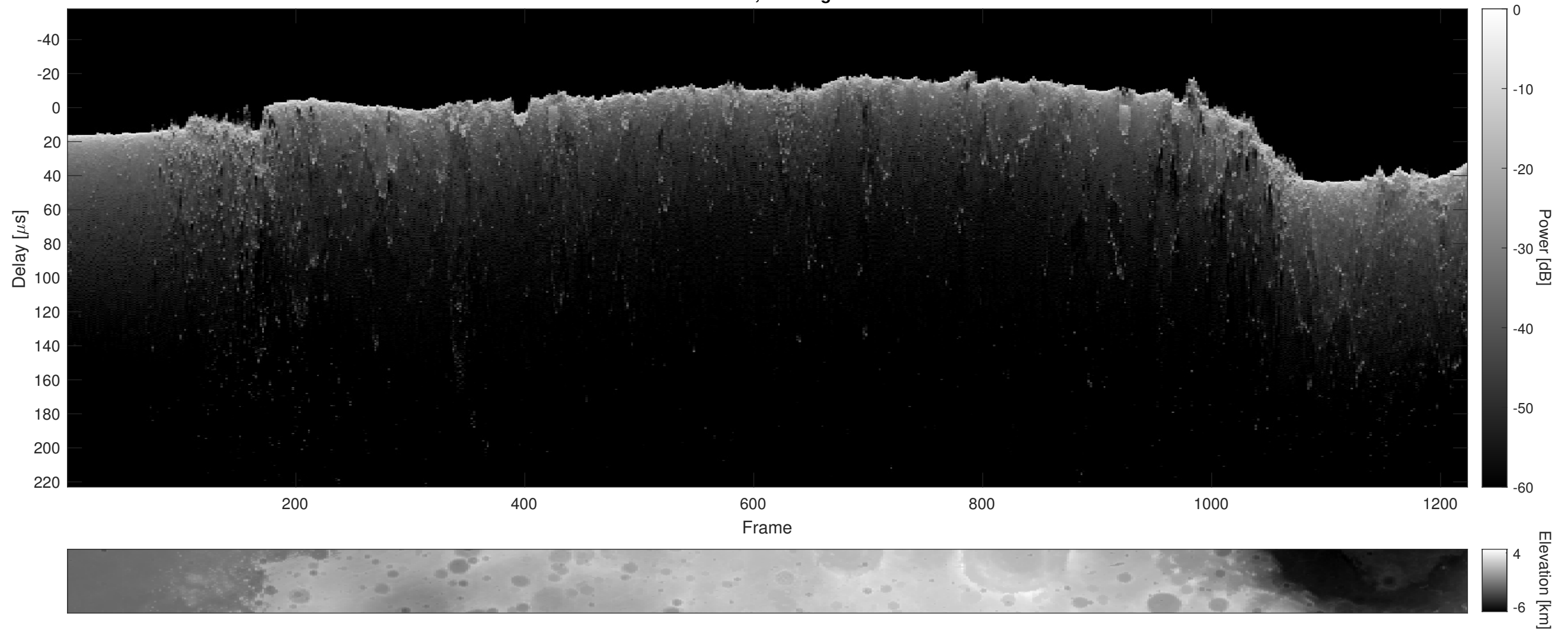
Orbit 7200, Cluttergram
