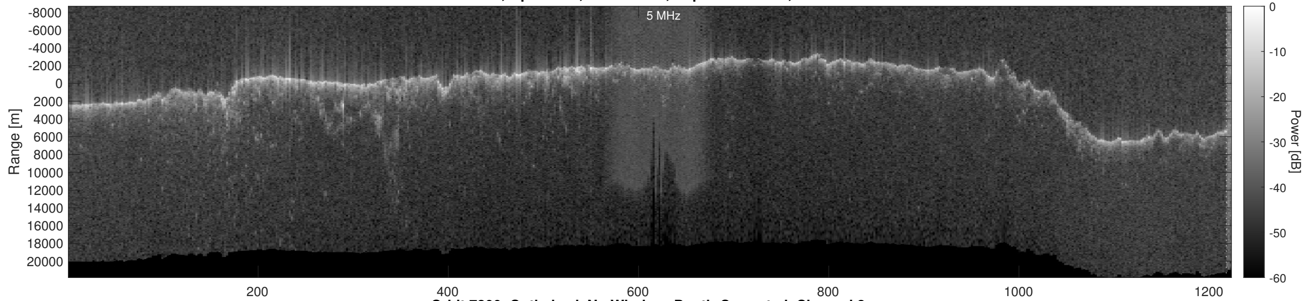
Orbit 7200, Optimized, No Window, Depth-Corrected, Channel 2
