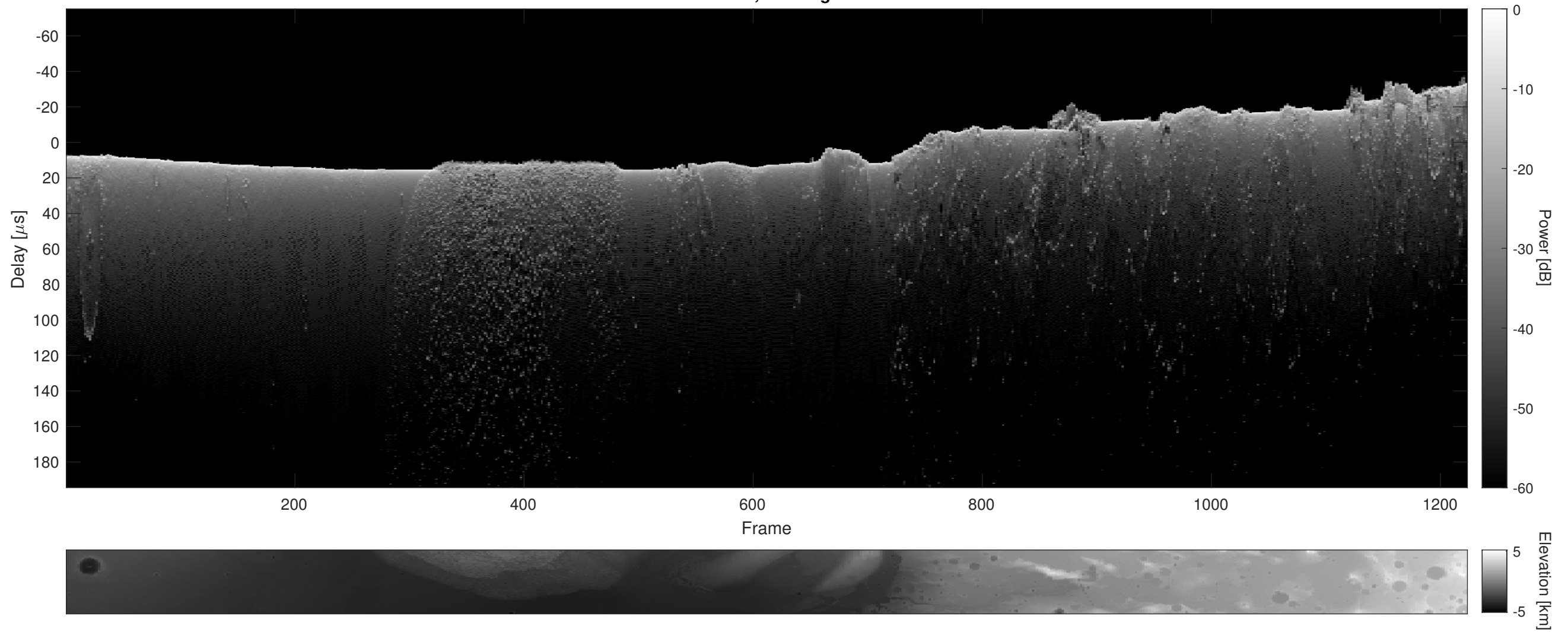
Orbit 7202, Cluttergram
