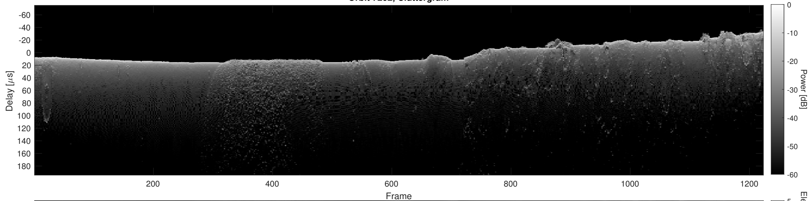
Orbit 7202, Cluttergram
