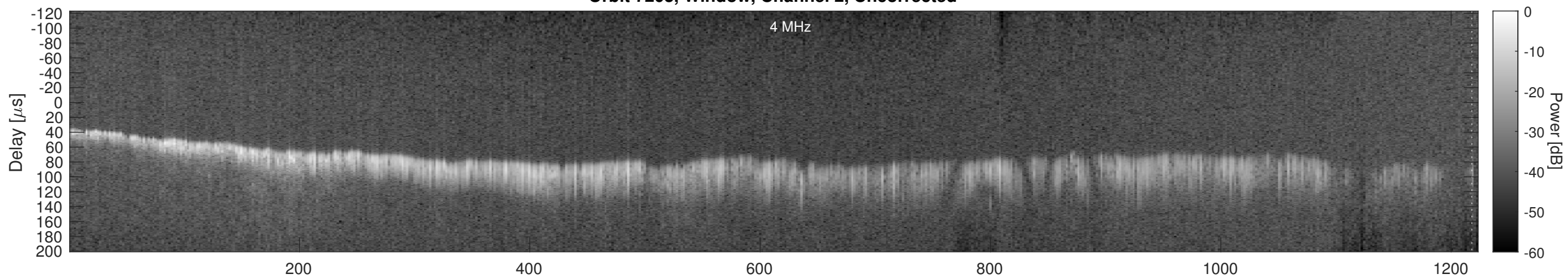
Orbit 7203, Window, Channel 2, Chapman
