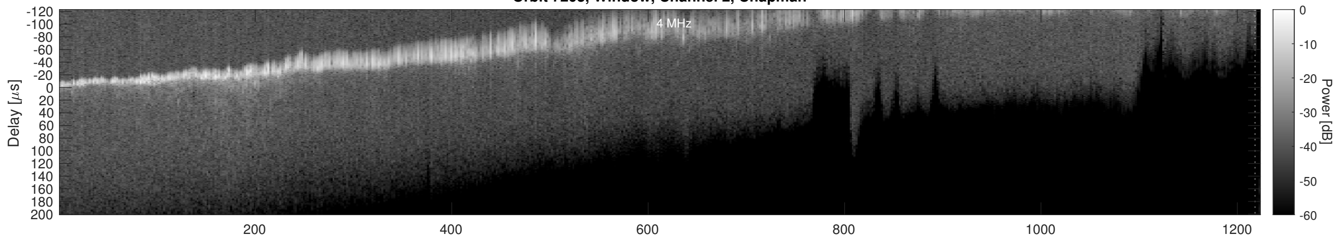
Orbit 7203, Window, Channel 2, Optimized
