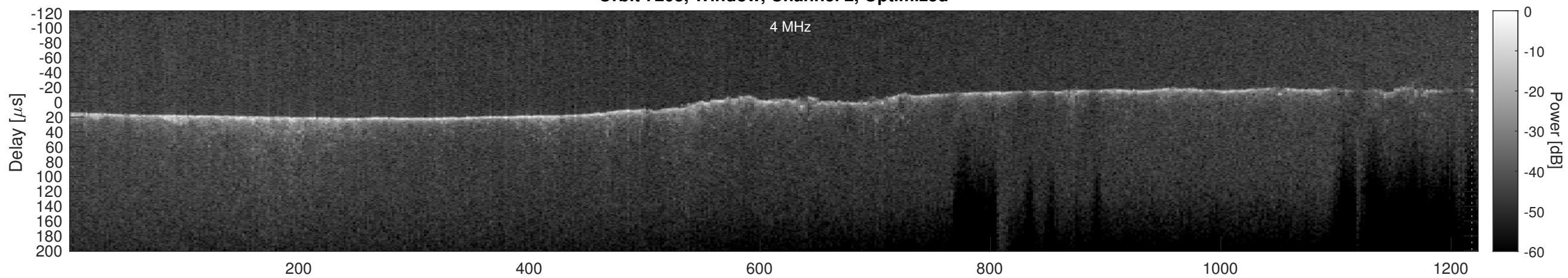
Orbit 7203, Cluttergram
