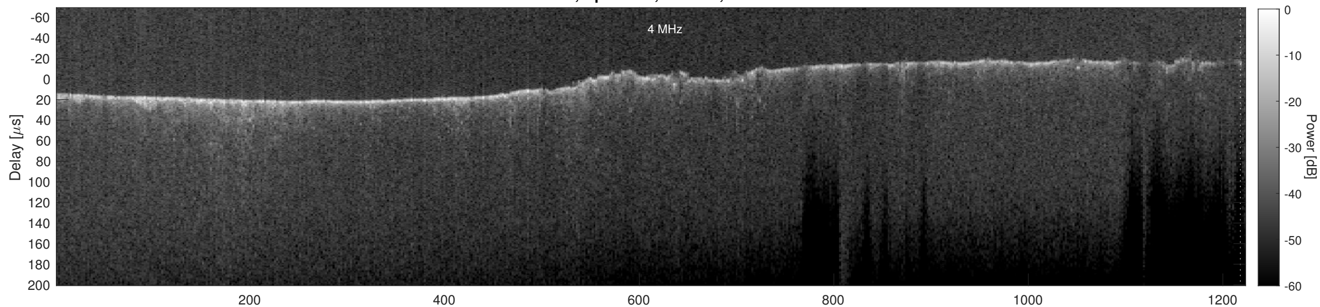
Orbit 7203, Cluttergram
