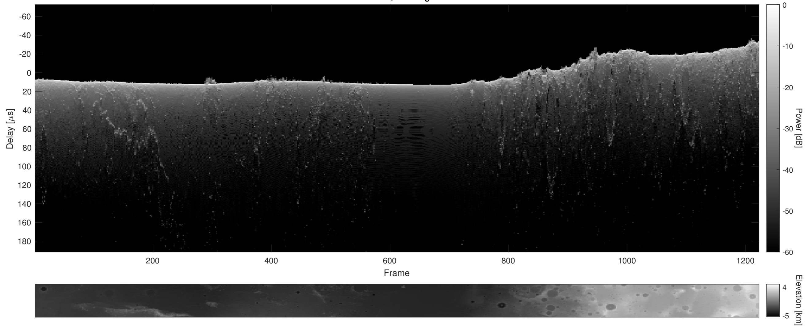
Orbit 7206, Cluttergram
