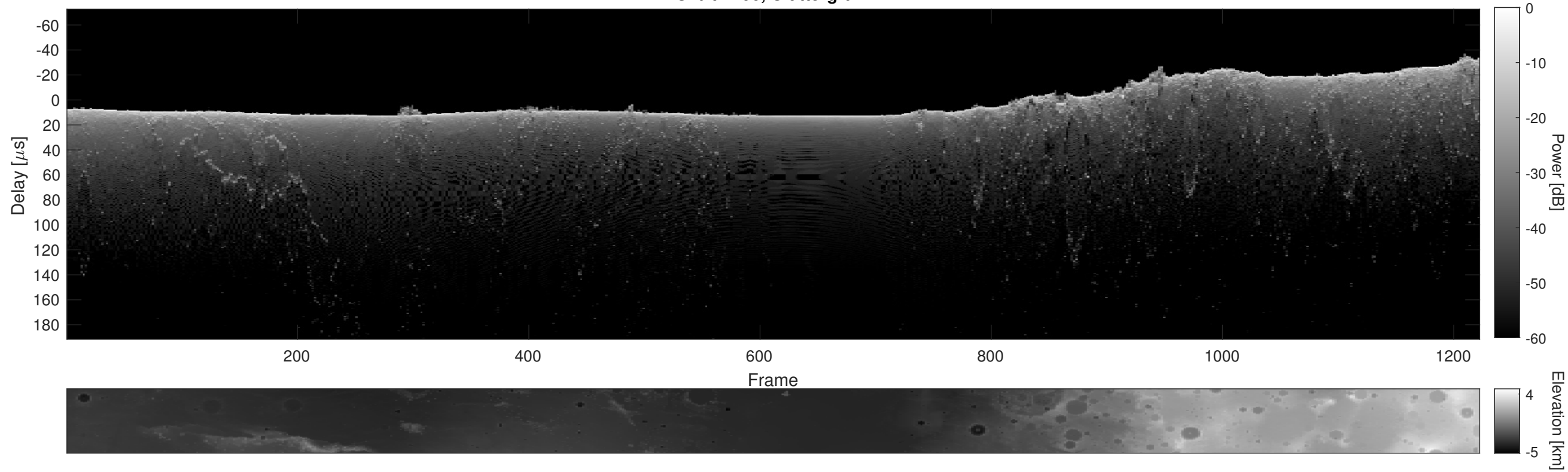
Orbit 7206, Cluttergram
