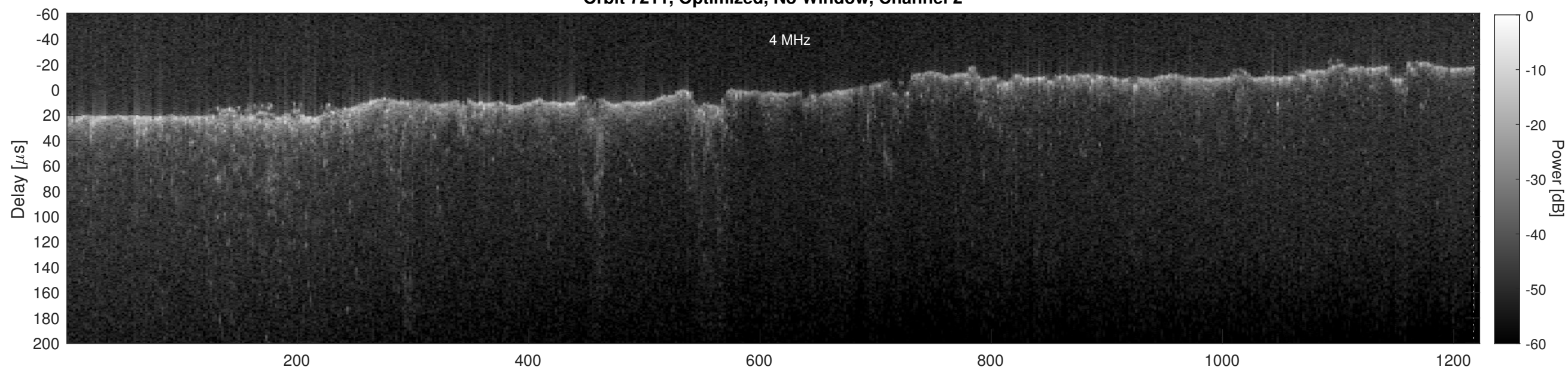
Orbit 7211, Cluttergram
