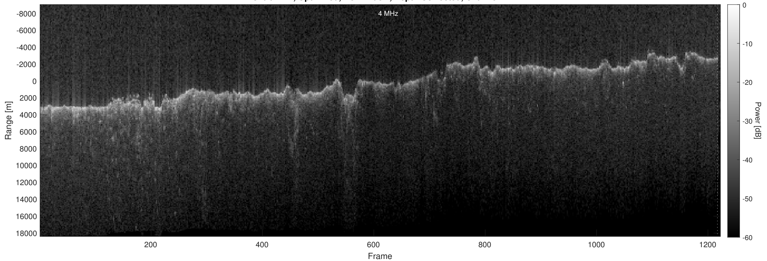
Orbit 7211, Optimized, No Window, Depth-Corrected, Channel 2
