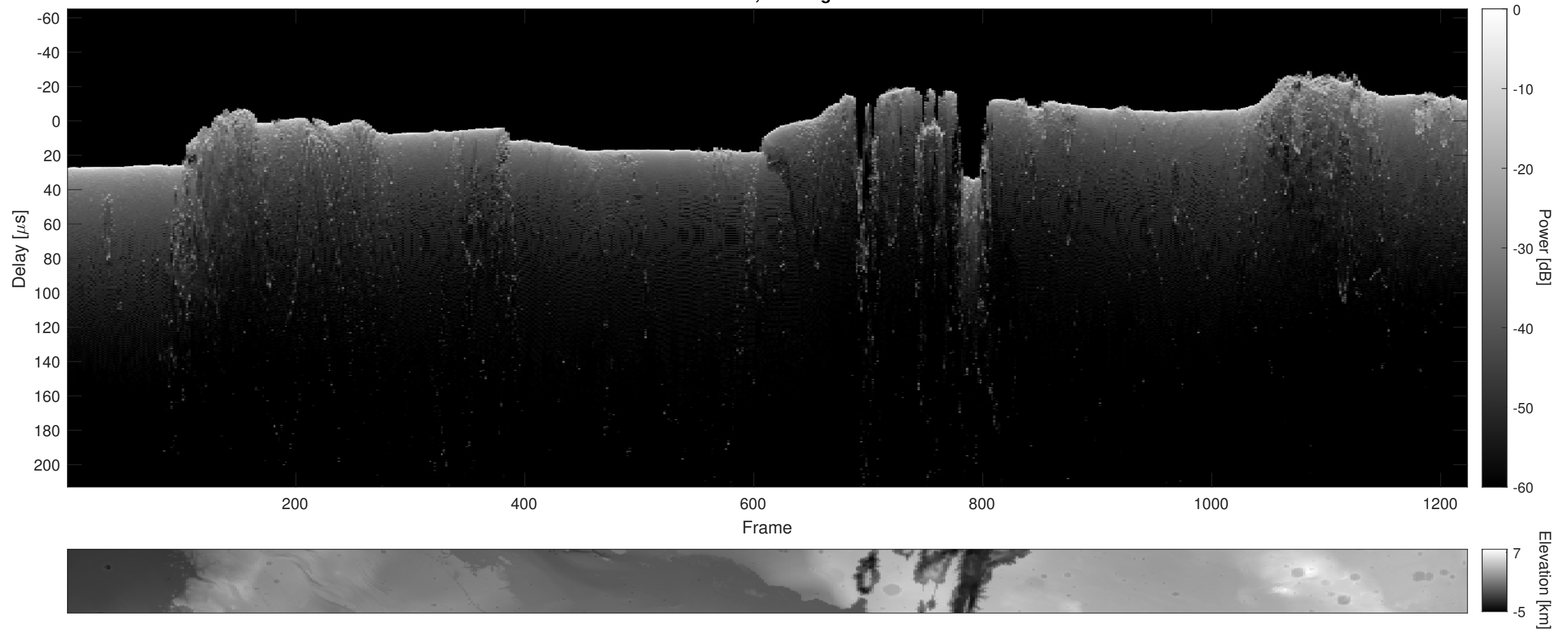
Orbit 7212, Cluttergram
