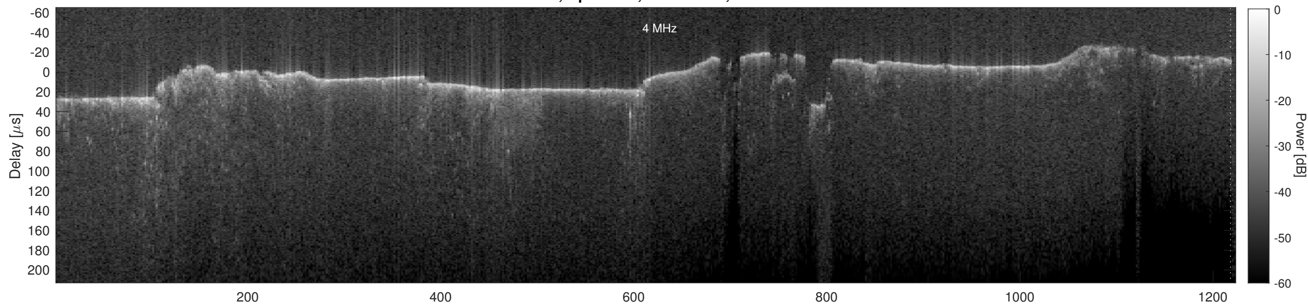
Orbit 7212, Cluttergram
