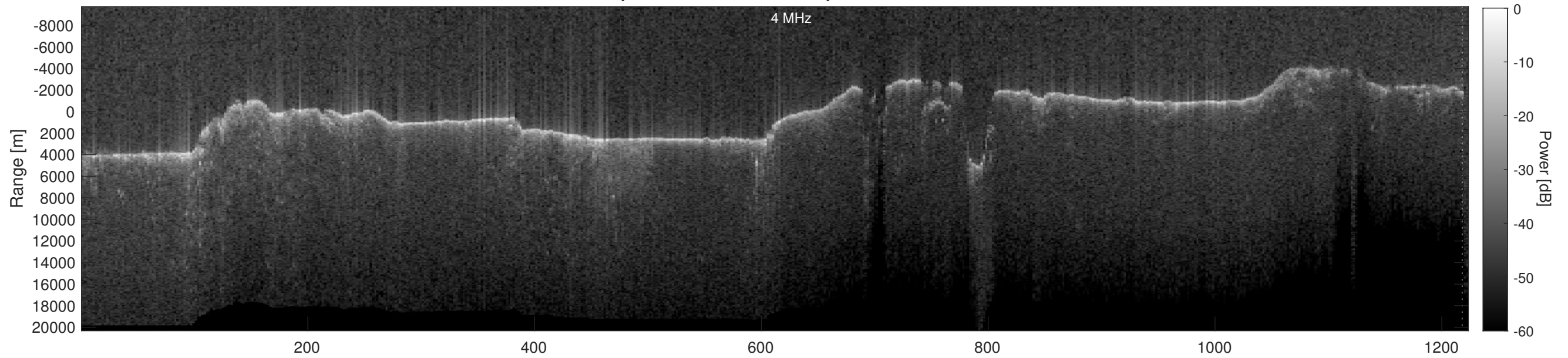
Orbit 7212, Depth-Corrected Cluttergram
