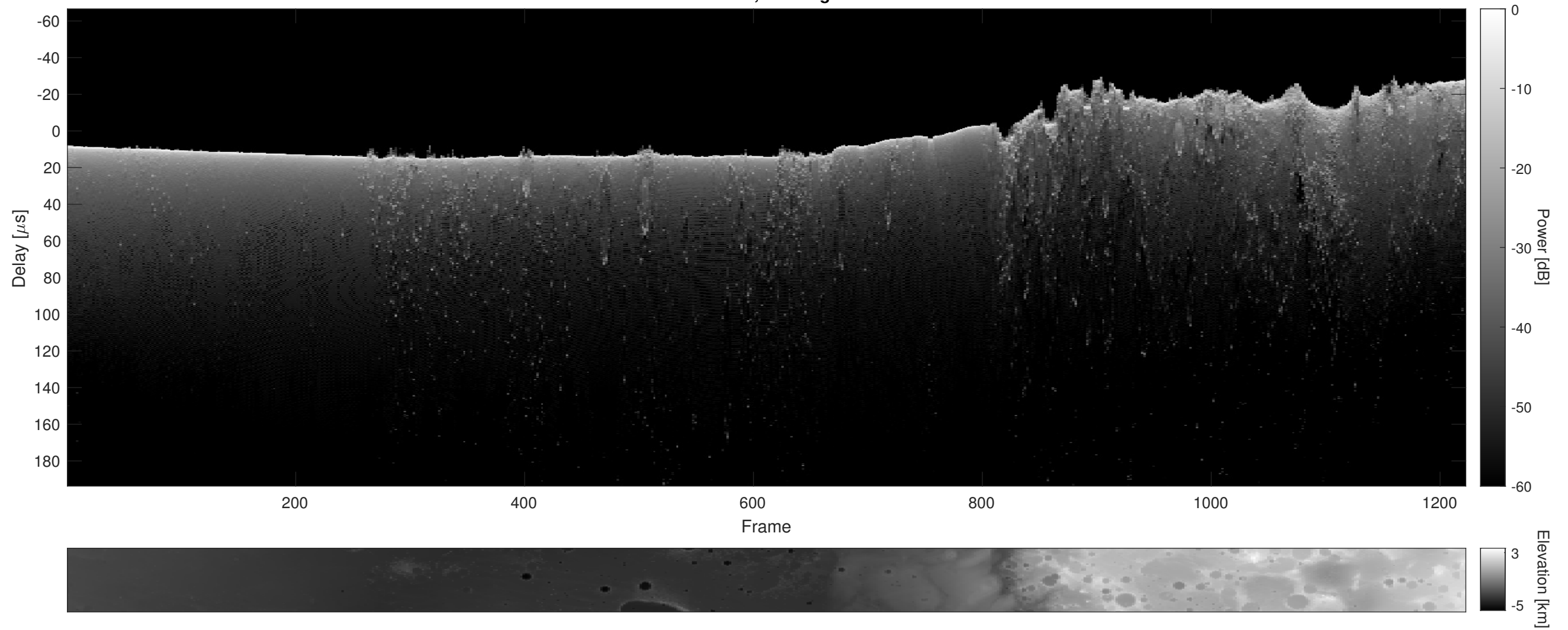
Orbit 7213, Cluttergram
