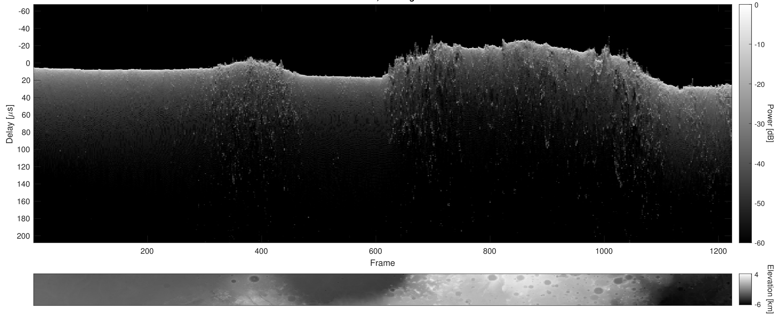
Orbit 7214, Cluttergram
