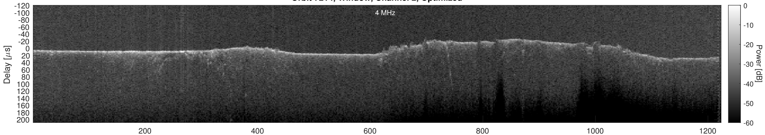
Orbit 7214, Cluttergram
