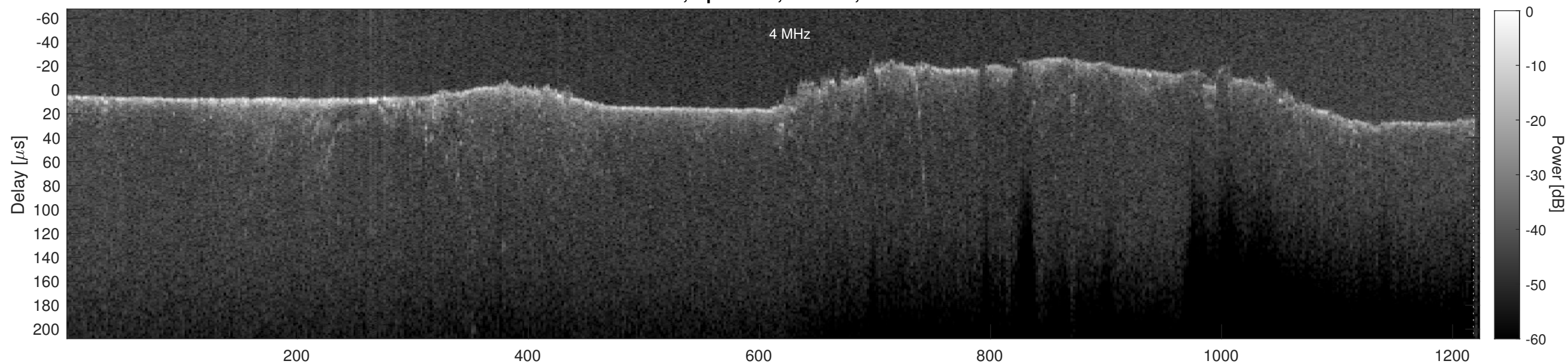
Orbit 7214, Cluttergram
