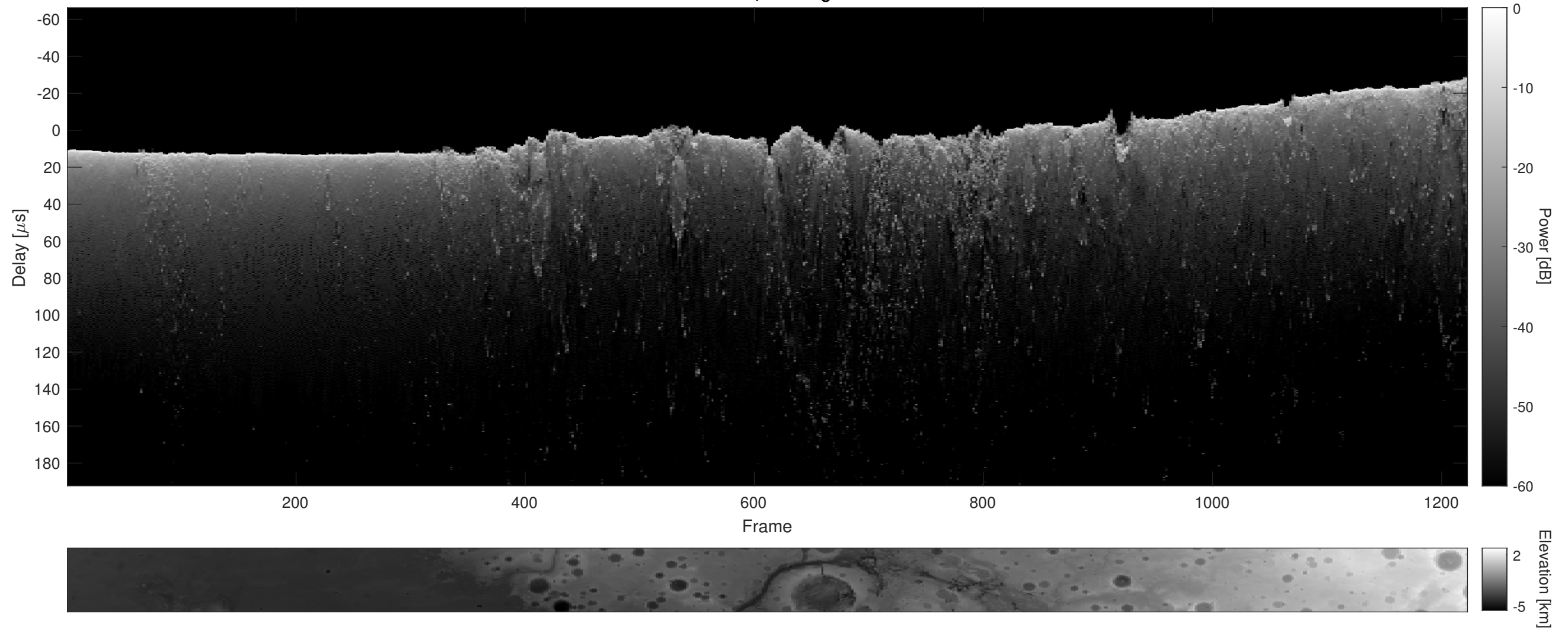
Orbit 7215, Cluttergram
