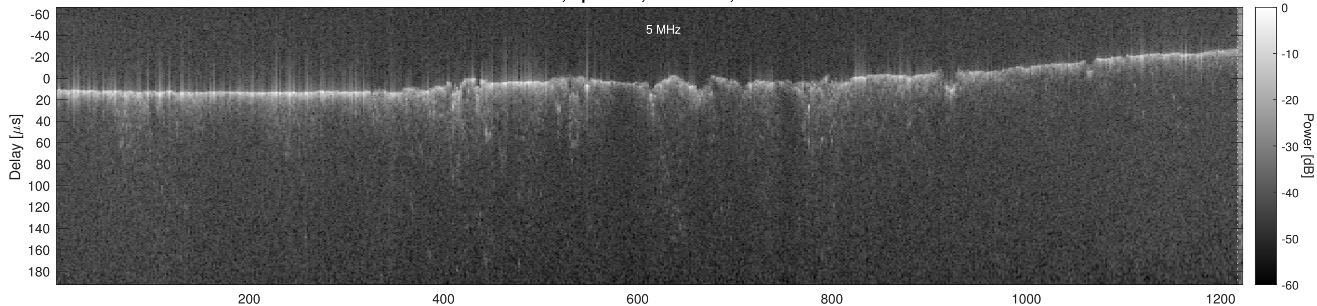
Orbit 7215, Optimized, No Window, Channel 2
