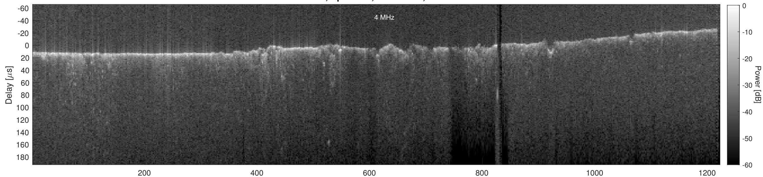
Orbit 7215, Cluttergram
