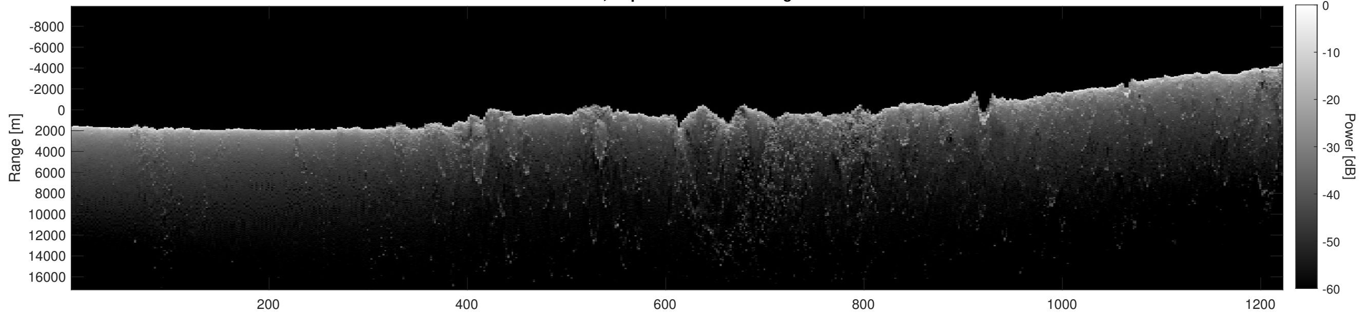
Orbit 7215, Depth-Corrected Cluttergram
